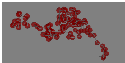
Edwards-Polymermodell
